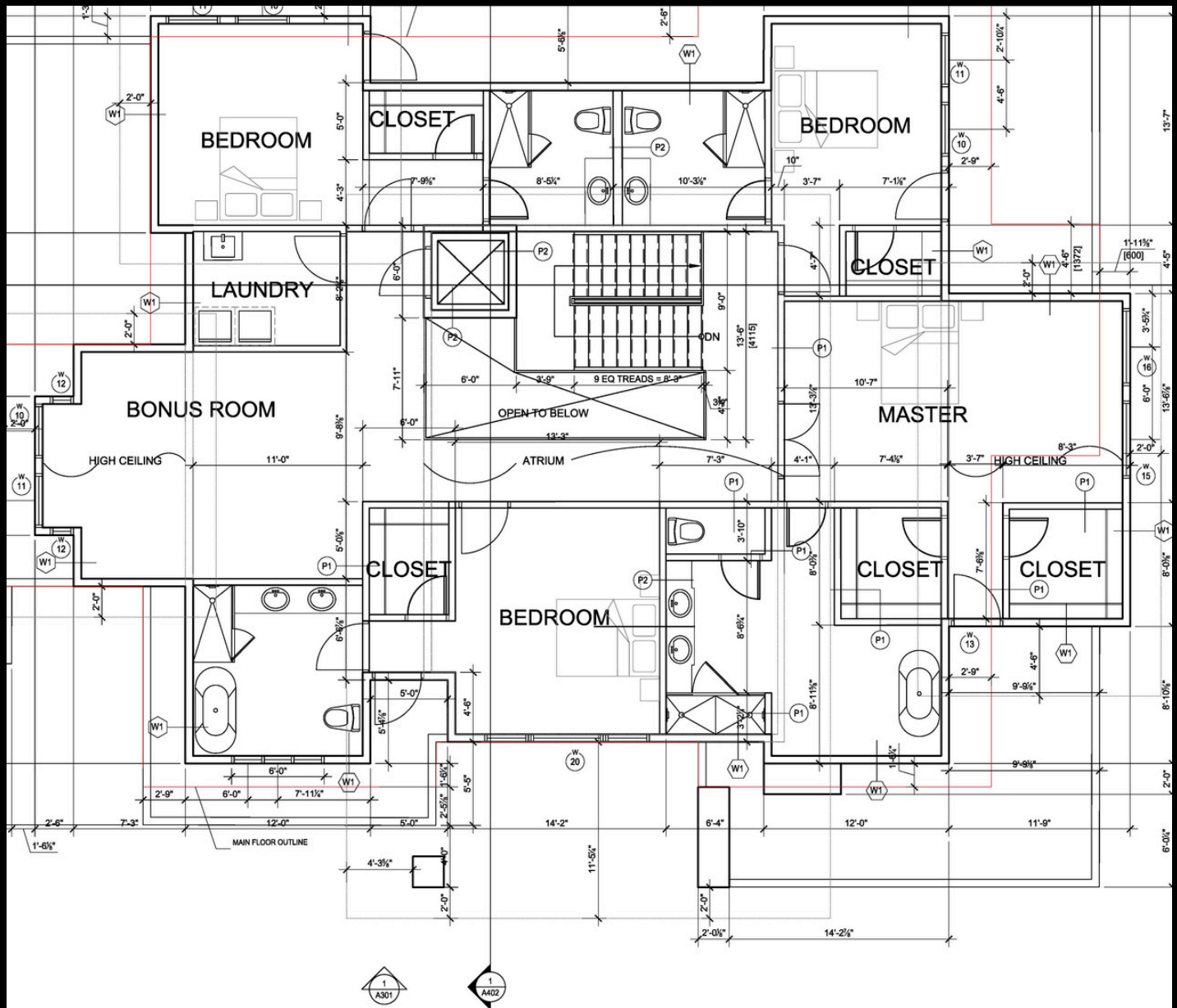
SECOND FLOOR 2550 SQFT
